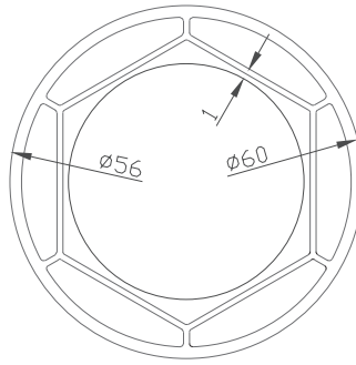
70 mm Boru 70 mm Pipe
