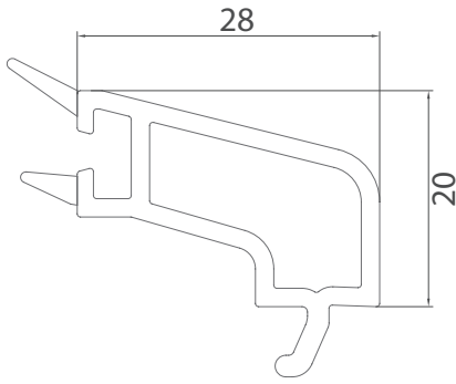
Dinamic 20 mm Çift Cam Çita Dinamic Double Glazing Bead 20 mm
