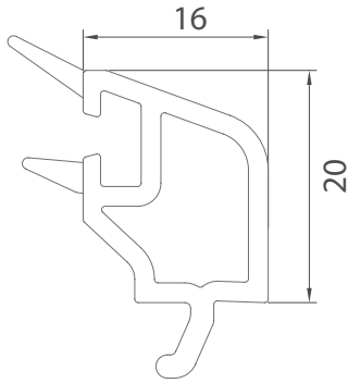
Momentum 24 mm Çift Cam Çita Momentum Double Glazing Bead 24 mm
