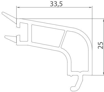
Energy 24 mm Çift Cam Çita Energy Double Glazing Bead 24 mm
