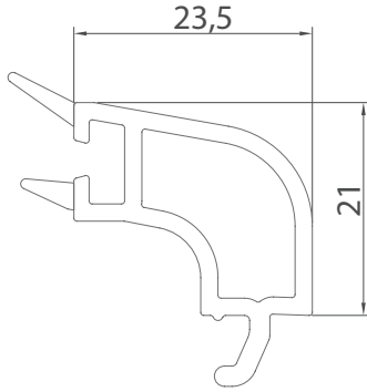
Dinamic 24 mm Çift Cam Çita Dinamic Double Glazing Bead 24 mm
