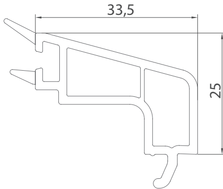
Energy 24 mm Çift Cam Dekoratif Çita Energy Double Glazing Decotative Bead 24 mm
