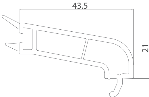
Dinamic 4 mm Tek Cam Çita Dinamic Single Glazing Bead 4 mm
